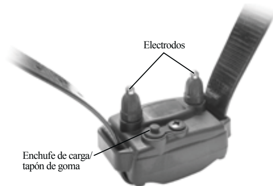
Collar receptor
