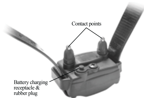
Receiver/Collar
